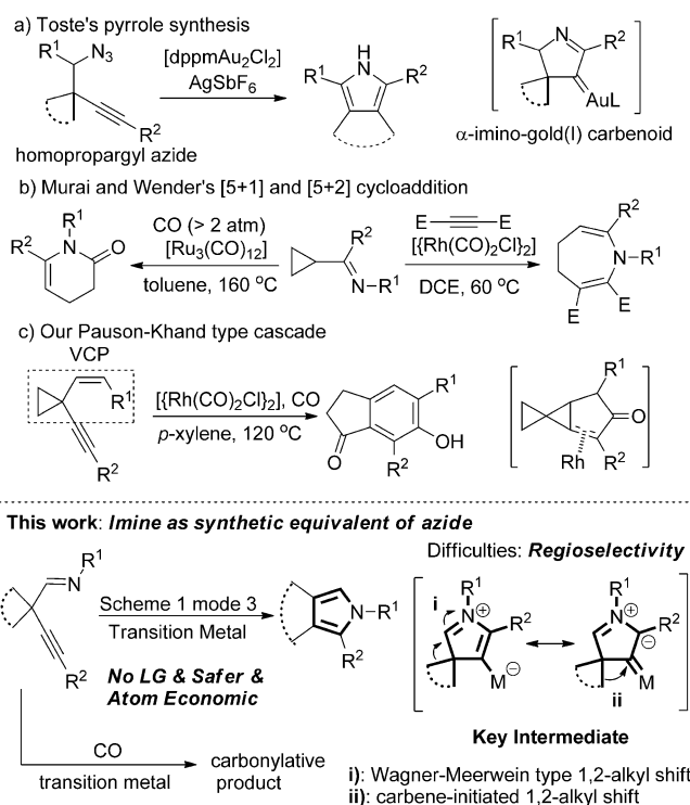
Scheme 2. Previous work and this work. dppm = bis(diphenylphosphino)methane, DCE = 1,2-dichloroethane.
